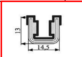
GC200 R-20 m
